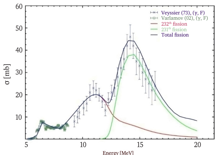
Figure 2. Dependence of the reaction cross-section on the excitation energy upon ^{232}\text{Th} nuclear photofission: circles and crosses – experiment, (\gamma, F) – blue, (\gamma, f) – red, (\gamma, nf) – green curves
